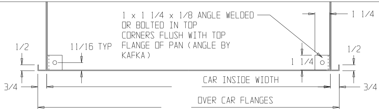
PLAN VIEW AT CAR TOP BEFORE GATE IS MOUNTED
